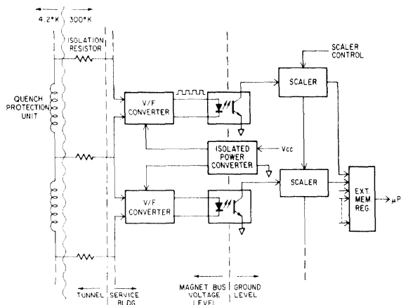
Fig. 4. Voltage Measurement Circuit.
