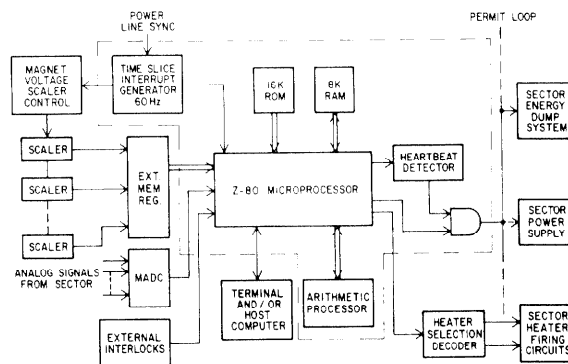
Fig. 3. Microprocessor System Block Diagram.
