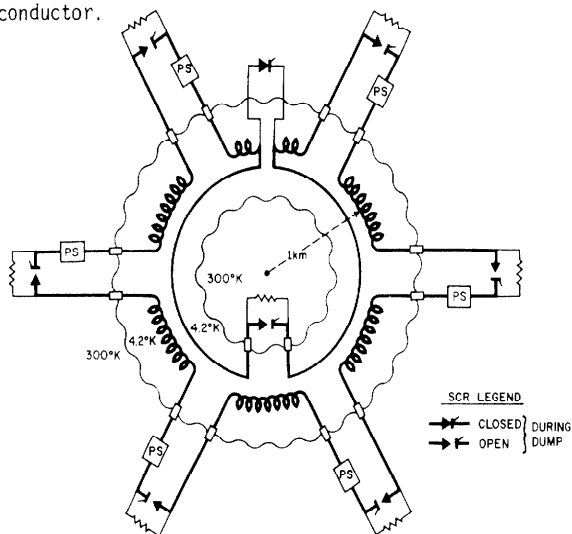
Fig. 1. Energy Doubler Magnet Circuit.
