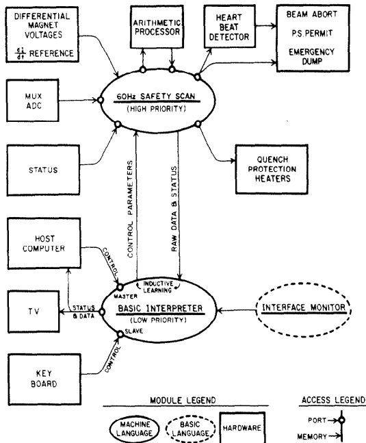
Fig. 5. System Communication Map.
