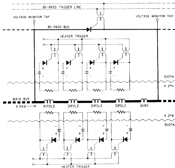
Fig. 2. Quench Protection Unit.
