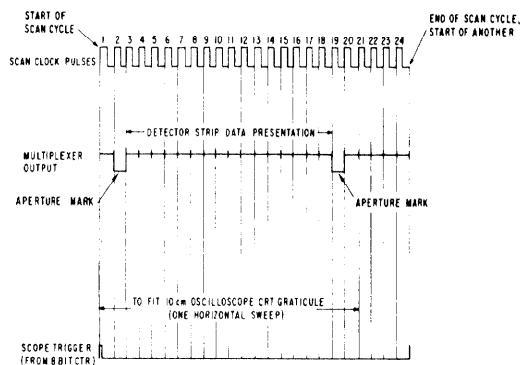
Fig. 3. Scanning sequence for data presentation
