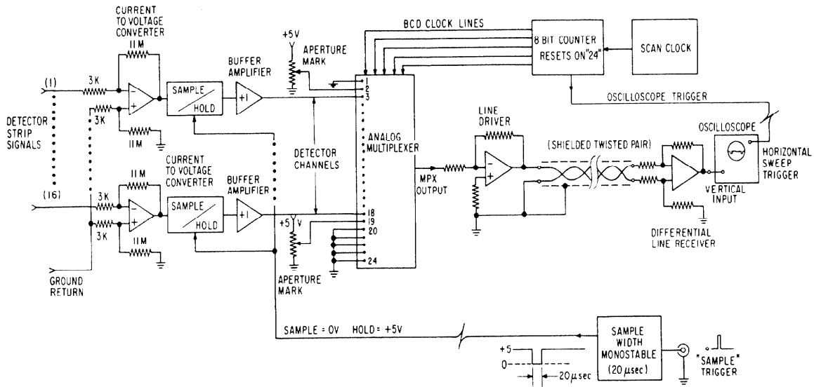
Fig. 2. Signal processing
