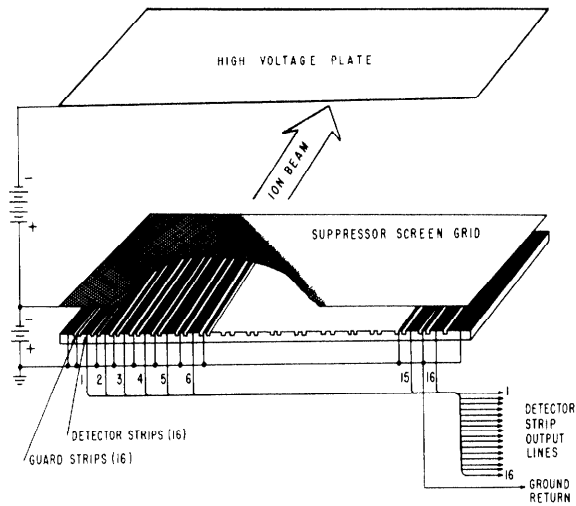
Fig. 1. Ion chamber positioned for horizontal beam size measurements
