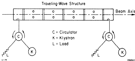
Fig. 2. System for using the same traveling-wave structure to accelerate both e^+ and e^- beams.
