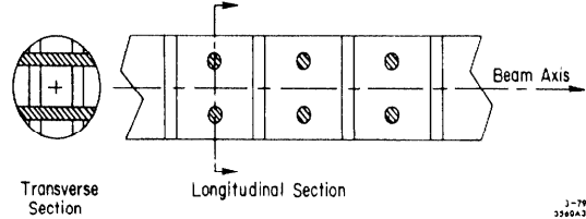
Fig. 3. Section of jungle-gym structure.
