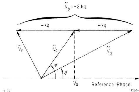
Fig. 1. Phasor diagram showing the superposition of the generator and beam-induced voltages for single-bunch beam loading.
