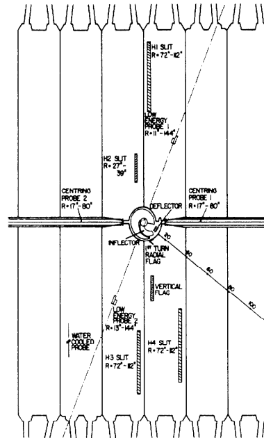
Fig. 1. Layout of diagnostic probes and defining slits in the central region. Two high-energy probes (not shown) operate between 144-320 in. along same azimuths as the low-energy probes.
