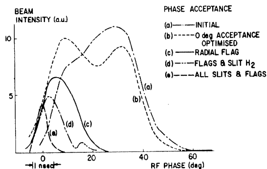
Fig. 3. Cyclotron phase acceptance to 500 MeV, measured by scanning the chopper phase at various stages of setting up for separated turns.
