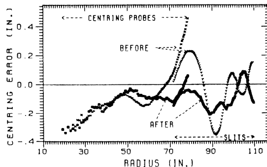
Fig. 2. Centring error along the dee gap (centring probes) and perpendicular to it (slits) before and after harmonic coil fitting.
