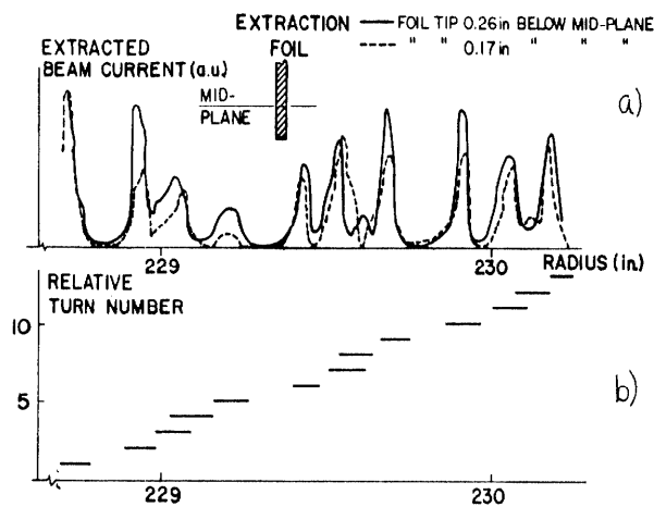
Fig. 5. Turn pattern (a) and the base width versus relative turn number (b) obtained by scanning the stripper foil near 200 MeV.
