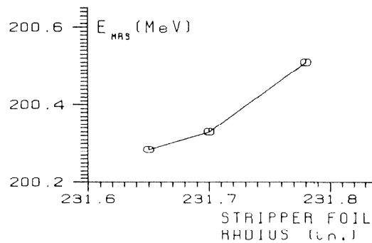
Fig. 6. Measured energy variation over a single turn.
