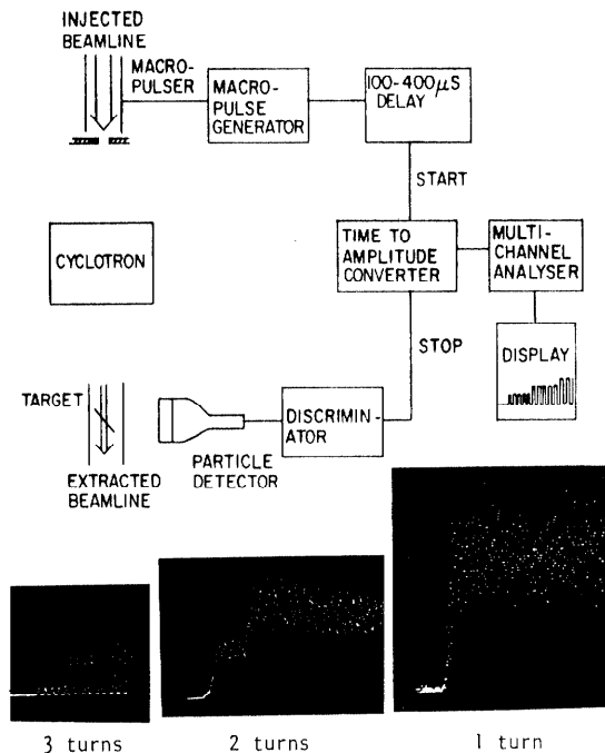
Fig. 4. Time-of-flight system and displays for multiple and single turn extraction.
