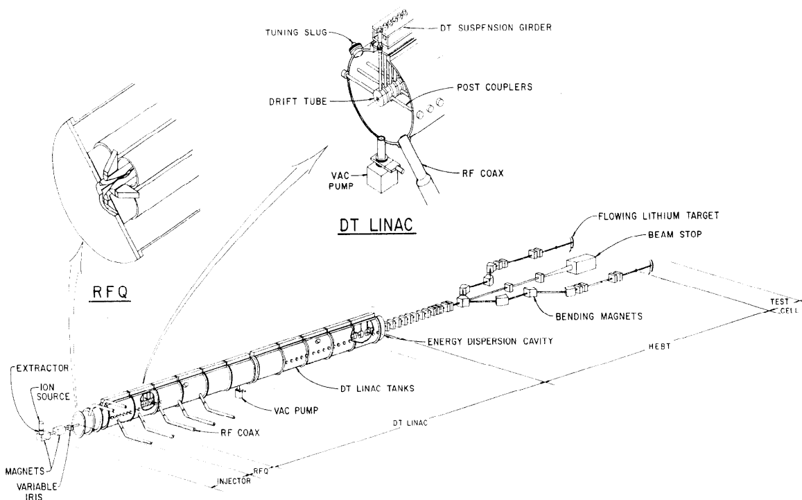
Fig. 1. Overall layout of the FMIT accelerator and beam transport system.
