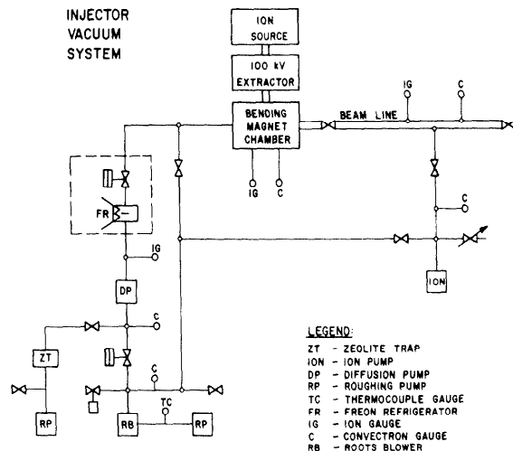
Fig. 1. The FMIT accelerator injector vacuum system.
