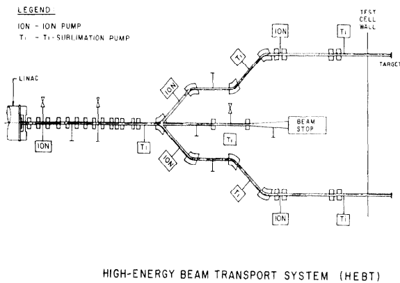
Fig. 3. The vacuum system for the High-Energy Beam Transport (HEBT) system for the FMIT Facility.
