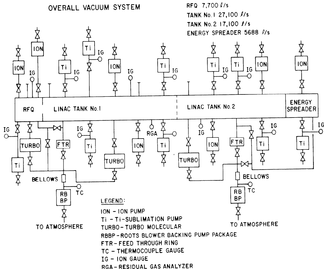
Fig. 2. The overall vacuum system for the FMIT accelerator.
