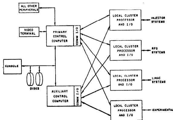
Fig. 11. Facility control system schematic.
