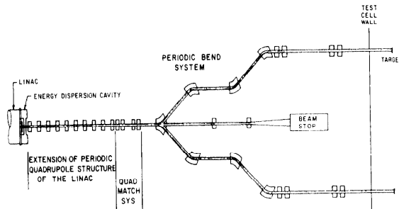
Fig. 10. High-Energy Beam Transport system.
