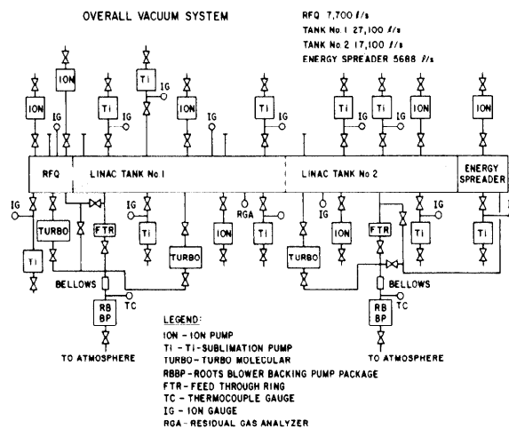
Fig. 8. Linac vacuum system.
