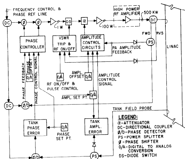
Fig. 9. RF system schematic.
