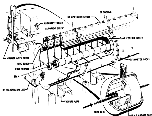
Fig. 7. Conceptual design of the drift-tube Linac tank and drift-tube support system.
