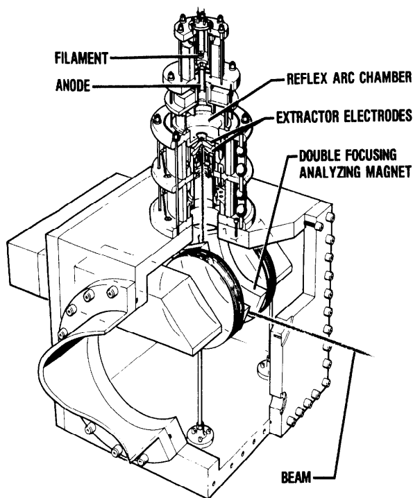
Fig. 6. Cutaway view of the ion source and extraction system.
