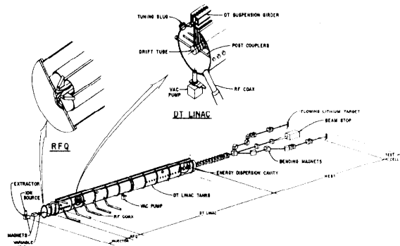
Fig. 3. Pictorial schematic of FMIT Linac components.
