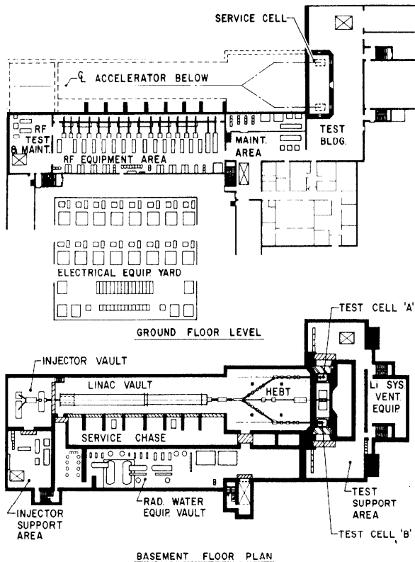
Fig. 2. FMIT Facility layout from Title I Design Study.
