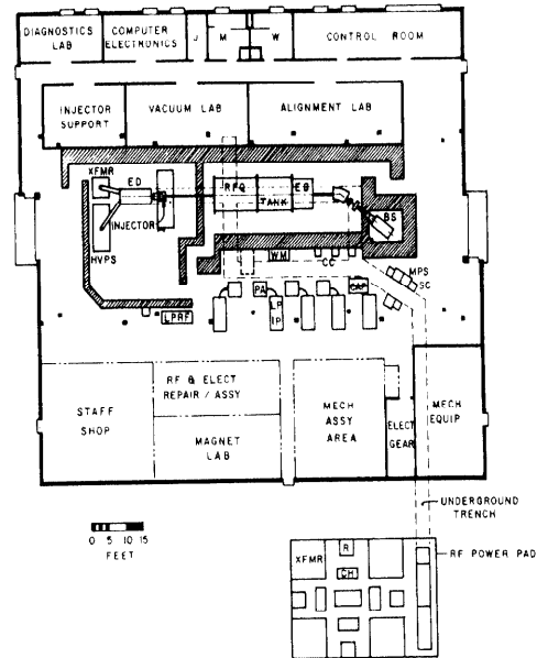
Fig. 5. FMIT prototype layout.
