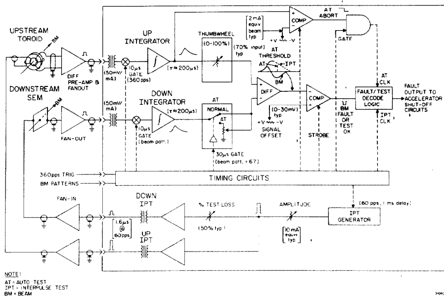
Fig. 3. Pulse-to-pulse comparator module.
