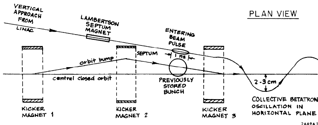
Fig. 2. Injection System Schematic.
