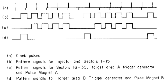
Fig. 2. Pattern signals for 60 pps OFF, 60 pps at BeV to area B, remainder at 20 BeV to area A.
