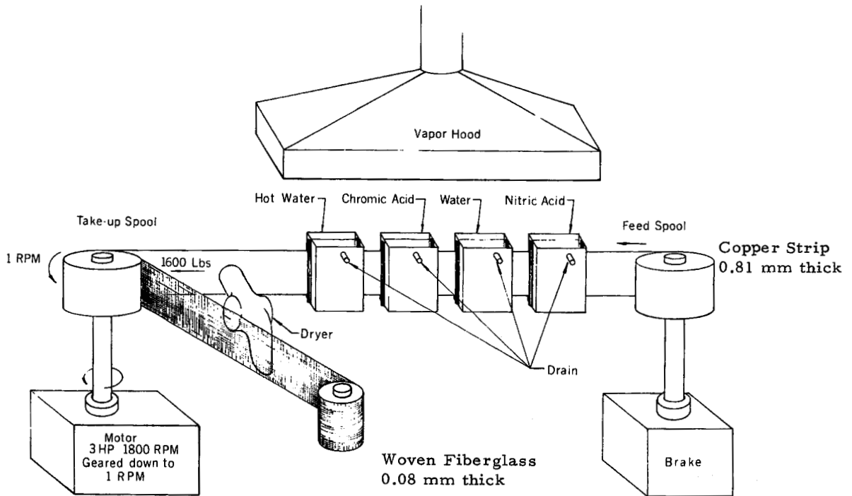
Fig. 3. Schematic of the coil winding process.
