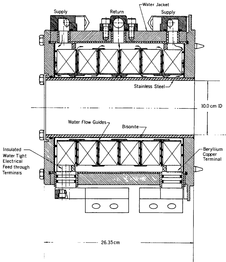
Fig. 1. Schematic of assembled solenoid.
