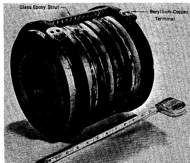
Fig. 5. Completed coil assembly.
