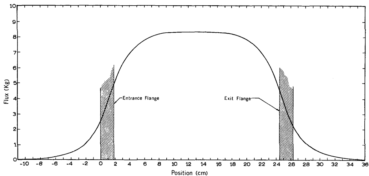
Fig. 6. Axial field profile.
