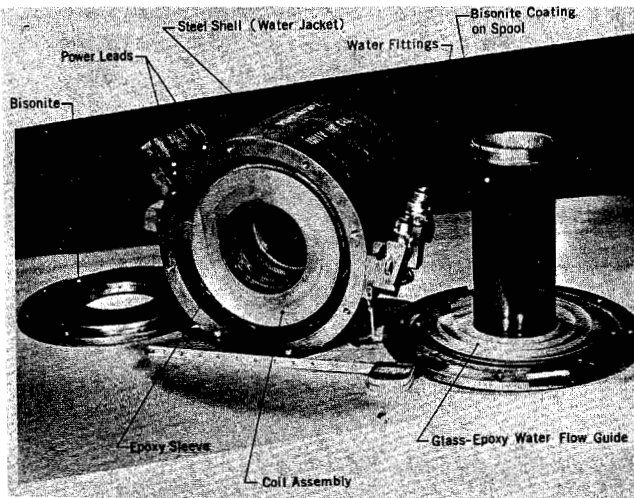
Fig. 2. Exploded view of solenoid.
