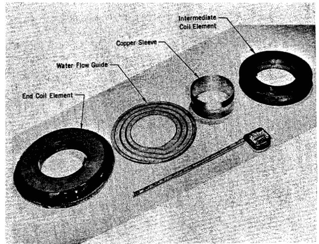
Fig. 4. Coil pair components.
