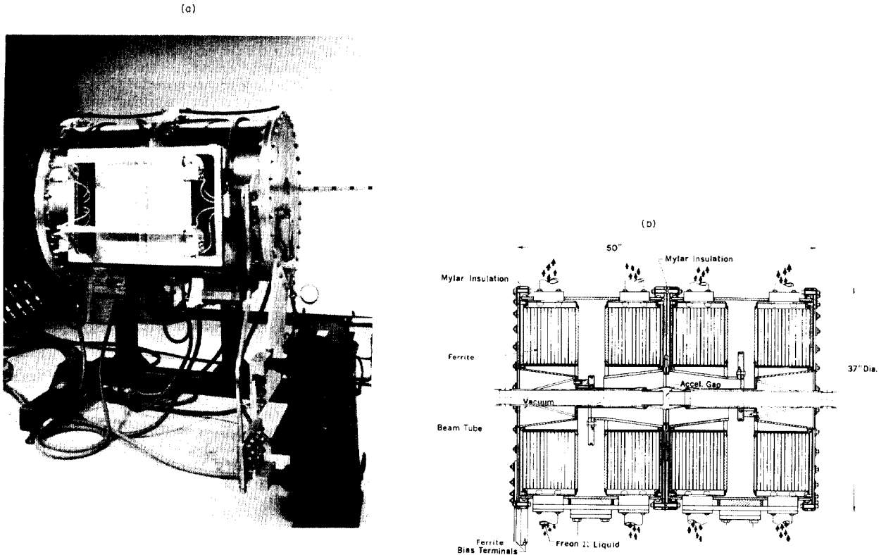
Fig. 1. (a) Prototype HF RF resonator. The resonator contains 30-in.-diam ferrite discs. The case carries the ferrite-bias current, which for the initial test was supplied by the transformer shown connected above. (b) Cross-section of the HF resonator. The output voltage of the two resonator sections are combined to excite a single accelerating gap. Freon-11 is circulated between the ferrite discs for cooling.
