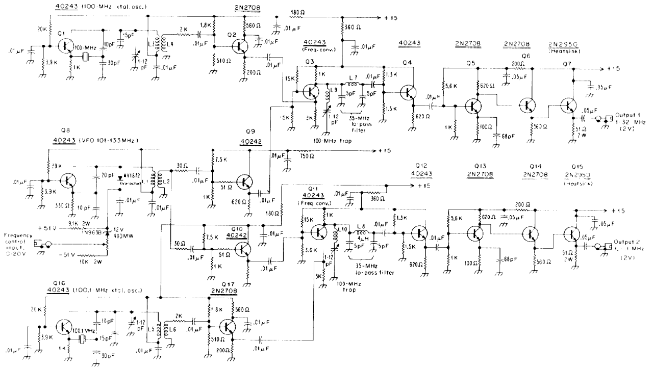
Fig. 4. Master-oscillator schematic. The master oscillator is a two-channel beat-frequency oscillator which produces an output frequency that is variable from 1 to 32 MHz. The frequency of the second channel is displaced from that of the first by 0.1 MHz. It is used for frequency conversion in instruments throughout the Omnitron.
