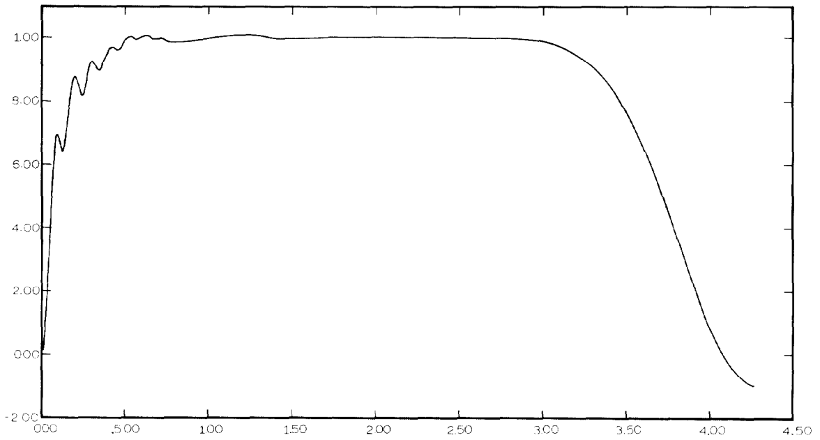
Fig. 6. Comparison of wave shape of magnetic field vs time, with a computer plot of the magnet excitation current vs time.
