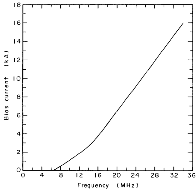
Fig. 2. Ferrite-bias current vs frequency for the HF prototype resonator.
