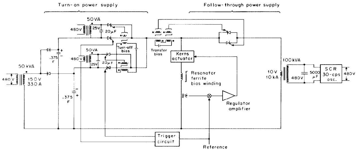
Fig. 3. Simplified schematic of ferrite-bias system. The ferrite bias uses two power supplies. A HV turn-on supply is used at the start of the sweep when the current is low and the inductance high. In about 1.5 ms, when the current reaches 1 kA and the inductance has dropped to about 5% of its unsaturated value, excitation is transferred to the low-voltage high-current follow-through power supply.
