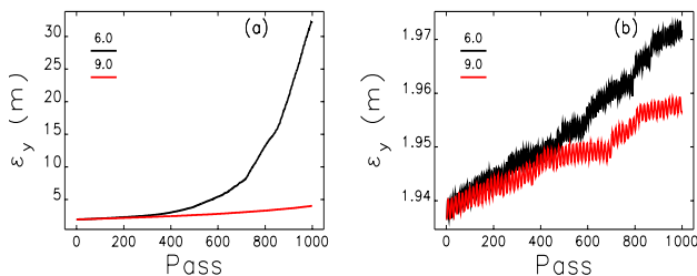
Figure 1: Emittance growth from equilibrium at different bunch lengths: (a) linear force model. (b) nonlinear force model.
