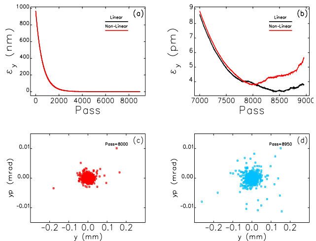
Figure 2: ILC damping ring positron beam emittance evaluation of entire damping cycle ( \sigma_z = 6 mm, 8962 turns): (a) entire cycle, (b) zoom in at the end of damping cycle, (c) particles phase space at Pass=8000, (d) particles phase space at Pass=8950 (before ejection, beam halo is formed).
