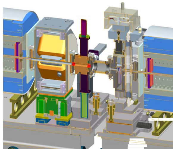
Figure 2: General layout of break between undulators.
