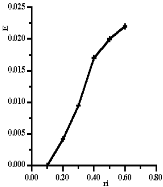
Fig.1: The dependence of space increment E of BCI on the ion beam radius r_i .
