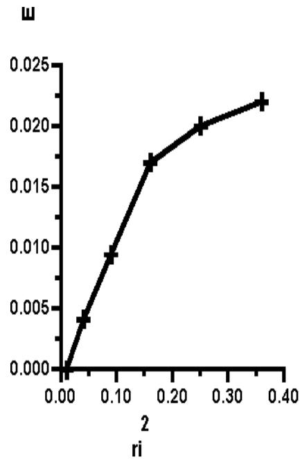
Fig.2: The dependence of space increment E of BCI on the ion beam radius r_i to square.
