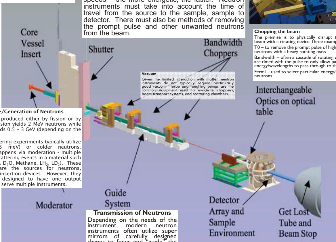
The MaNDi instrument at the Spallation Neutron Source at Oak Ridge National Laboratory. Image courtesy of Scott Keener.
