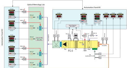
Figure 6: Optical Metrology Lab automation diagram
