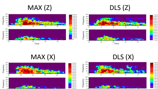
Figure 3: Frequencies excited by external impact and dissipation over time.
