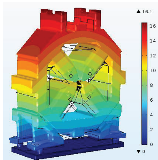
Figure 6: Total displacements ( \mu\text{m} ) in a 3D quadrupole heated by coils.
