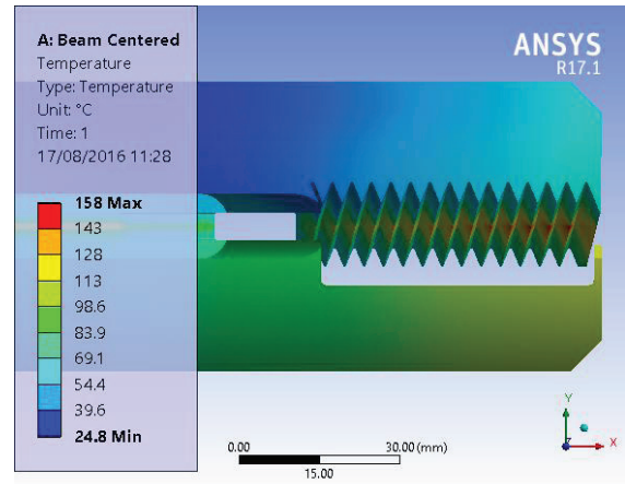
Figure 6: Temperature Plot CH9-1-2 Absorber.
