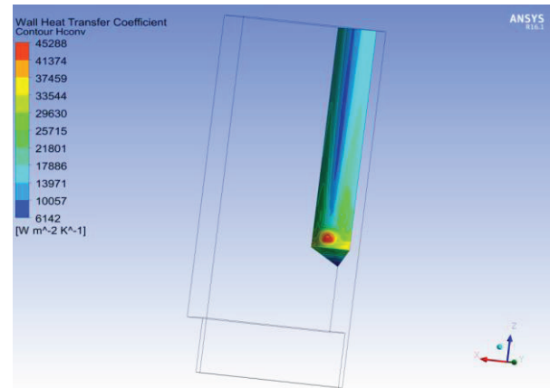
Figure 5: Heat Transfer Coefficient of a Cooling Channel.
