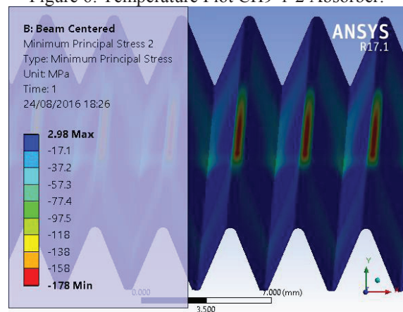
Figure 7: Minimum Principal Stress CH9-1-2 Absorber.
