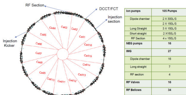
Figure 1: General storage ring vacuum layout.
