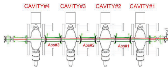
Figure 4: Injection section layout.
