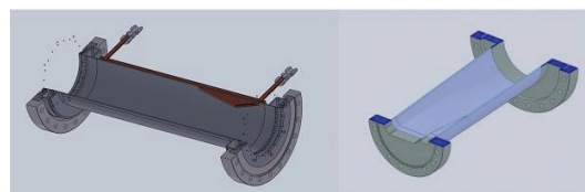
Figure 5: RF section layout, transition centre absorber and the upstream transition parts.
