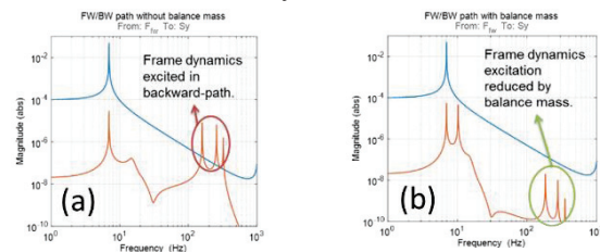
Figure 2: Transfer function for pitch correction in the 2 nd crystal of the DCM: forward path in blue and backward path in red. In (a) the reaction force acts against the long stroke frame, whereas in (b), against the balance mass.
