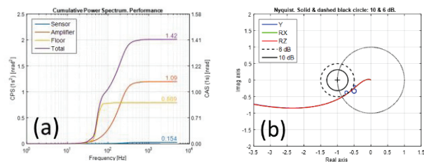
Figure 3: (a) Cumulative Power Spectrum Performance, analysing disturbances individual contributions. (b) Nyquist plot example, with analysis made for misalignment impacts on stability.
