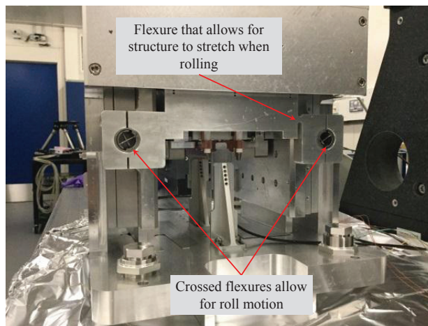
Figure 10: ML1 assembly at Diamonds Precision Metrology Lab (PML) [2].
