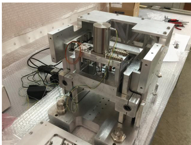
Figure 5: ML1 subassembly partially assembled.
