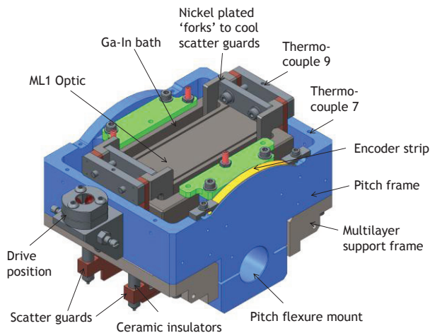
Figure 6: ML1 multilayer pitch assembly.
