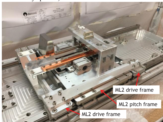
Figure 12: ML2 subassembly.
