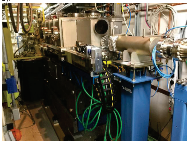
Figure 1: DMM installed in I02 optics cabin.
