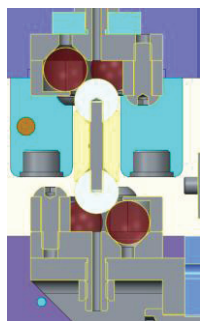
Figure 7: Section of stainless ball on nest of ruby balls.
