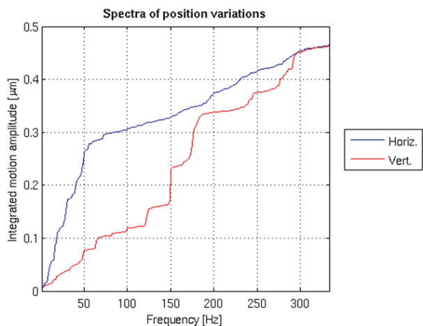
Figure 18: Integrated (RMS) position from 1-350Hz.
