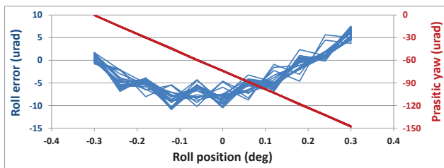
Figure 11: Parasitic pitch and yaw from roll axis [2].
