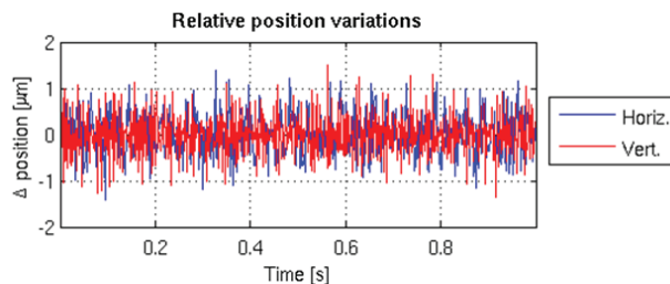
Figure 17: Beam vibration data.
