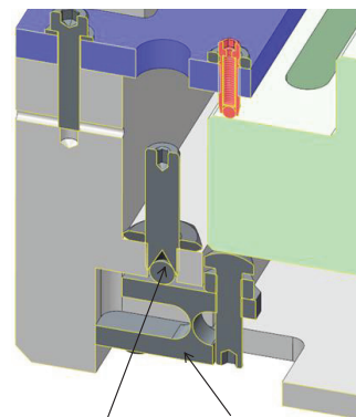
Figure 13: ML2 flexure adjusters.
