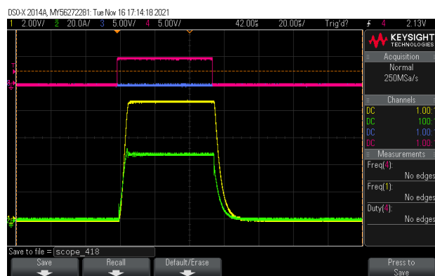
Figure 2. Pulsed Cathode Voltage, 105kV (scale 12kV/V), 55 \mu s pulse width and 400 Hz repetition rate.
