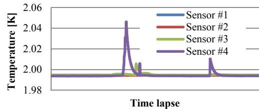
Figure 8: Temperature profile of cavity #1 during rf test.
