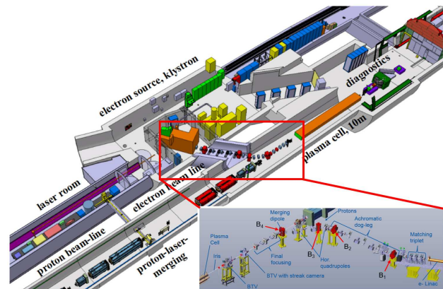
Figure 1: AWAKE tunnel and current electron beamline.
