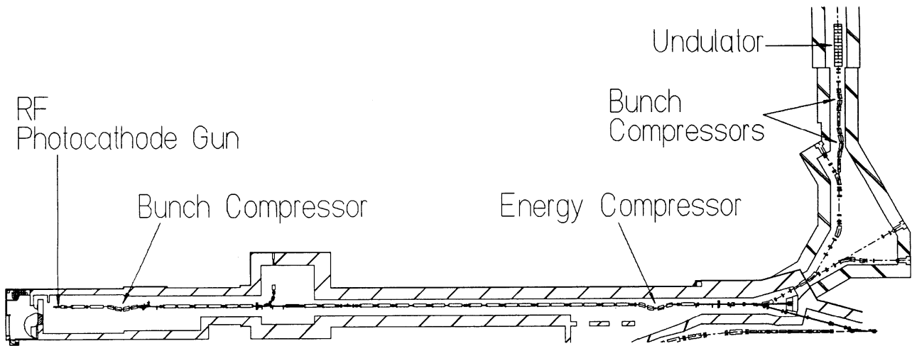
Fig.4 Schematic drawing of layout for SASE
