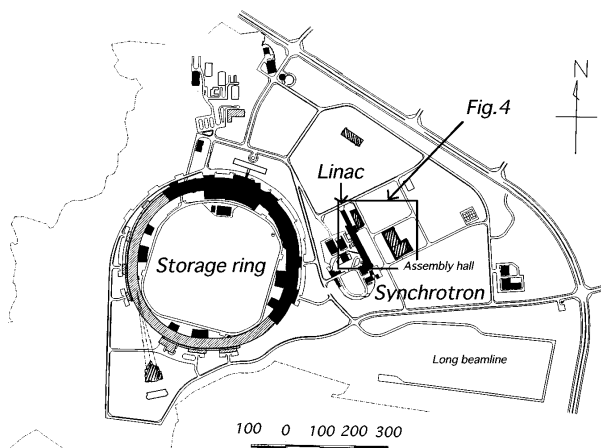
Fig.1 SPring-8 site layout
