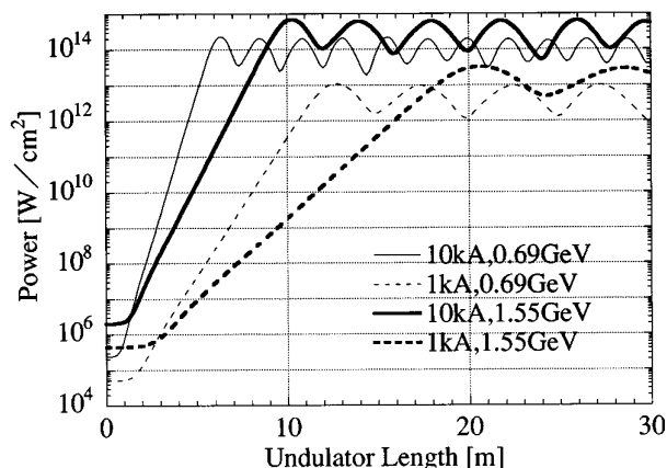
Fig. 2 Power growth in undulator
