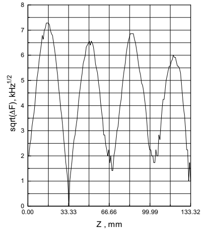
Fig.2. E r field distribution versus position of the disk bead on the axis of structure SBLC DLW with 2a=31.02mm (Θ=π).
