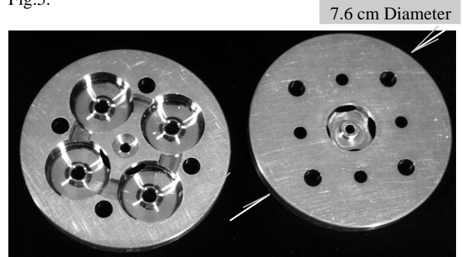
Fig.5. Manufactured X-band Cavity
