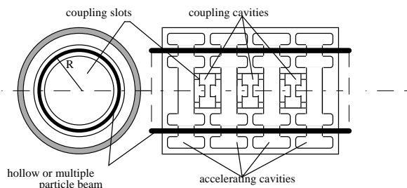
Fig.1. Magnetically Coupled MBS.
