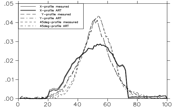
Figure 5: Beam projection on x, y, and 45 degree planes.
