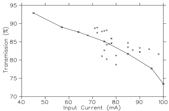
Figure 2: RFQ transmission as a function of input current. The solid line indicates the simulation and crosses the measured values.
