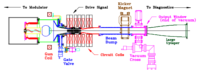
Fig. 1. The gyrokylystron test bed.
