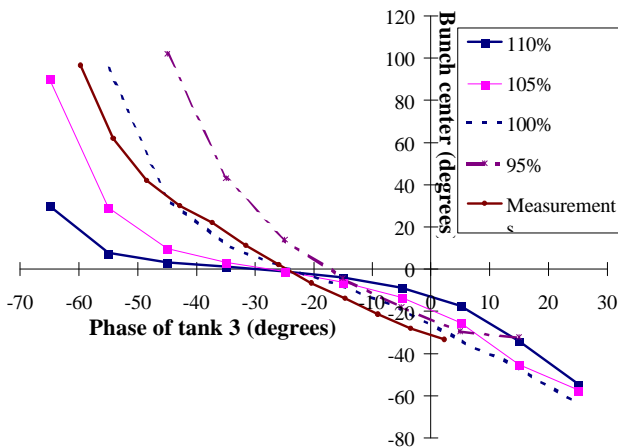
Fig. 4. Bunch centre as a function of protons arrival phase in tank 3. The experimental curve has been arbitrarily placed on this graph.
