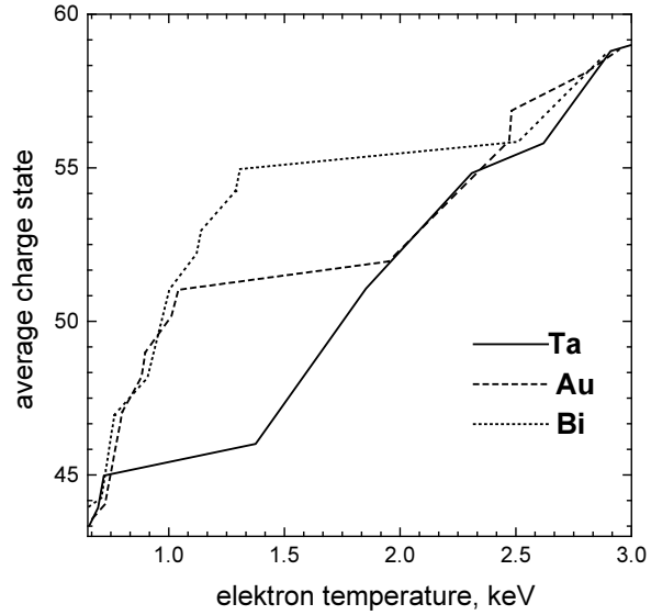
Figure 2: Calculated mean charge of Ta , Au and Bi dependent on the electron temperature
