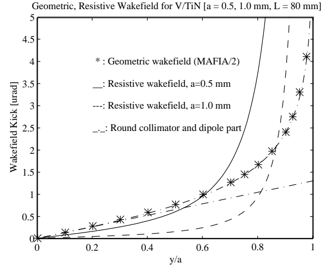
Fig. 3: Geometric and resistive wakefield estimates.
