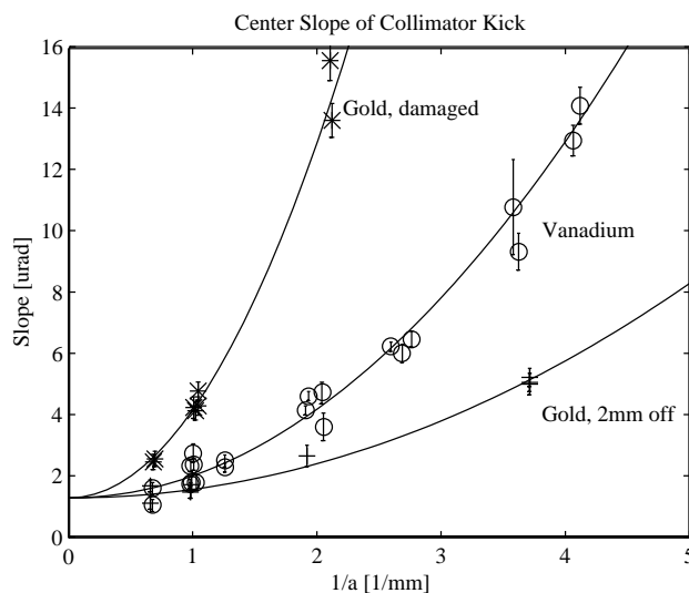
Fig. 5: Slope of the linear part of the wakefield kick versus 1/a . The fit (solid) shows a kick about a factor of 4 higher than expected for the resistive wakefield.
