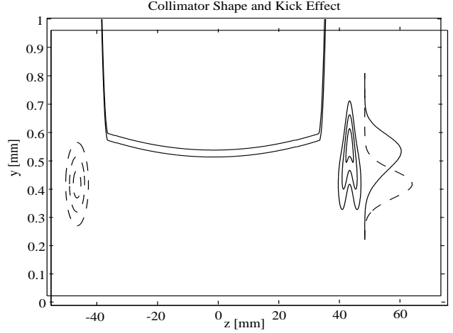
Fig. 2: Tapered collimator and a resultant wakefield kick of 3\sigma_y . The contour lines and projections of the incoming (dashed), and outgoing beam (solid) are shown.
