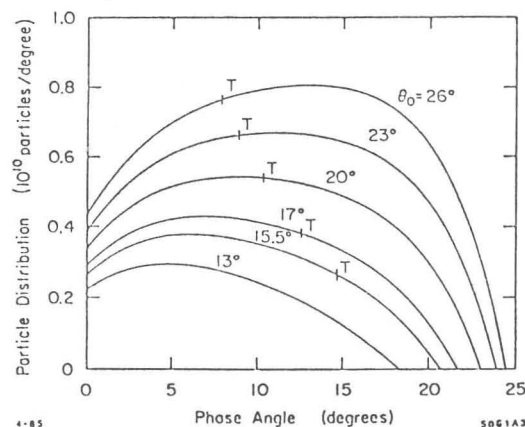
Figure 1: Linac Bunch Distributions [3]
