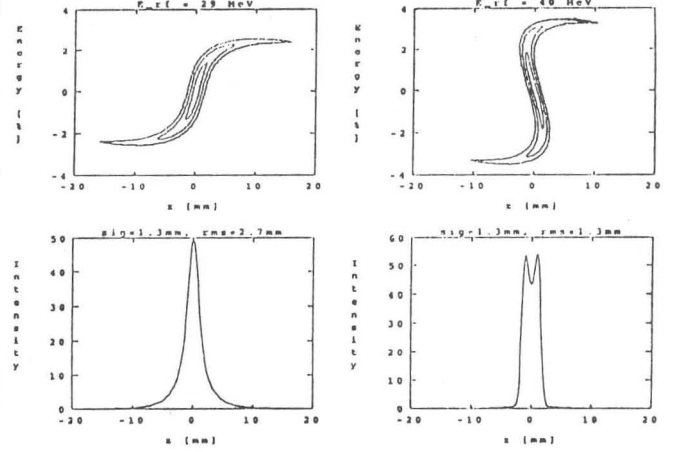
Figure 2: Under- and Over-Compression of the RTL Bunch Length
