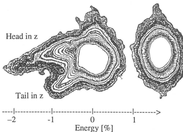
Figure 5: Beam Distributions at a Dispersive Point
