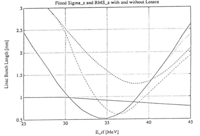
Figure 3: Bunch Length versus Compressor Amplitude
