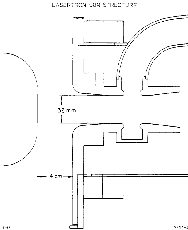
Fig. 2. The lasertron gun structure. The beam is confined against defocusing electric fields from the gun geometry and space charge by a longitudinal magnetic field of about 2000 gauss. The field on the cathode is about half the field at the cavity center causing a radial compression of the beam.
