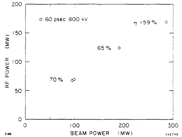
Fig. 6. Calculated power and efficiency for the SLAC proof of principle lasertron at 800 kV. This is too high a voltage for the electrode structure to hold off DC, but it may be possible to hold off using a short pulse.
