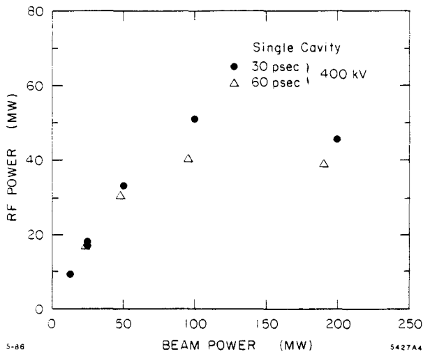
Fig. 4. The MASK calculated SLAC lasertron output power for various beam powers and for two optical pulse lengths. These results were obtained using a model with a single gap output cavity.
