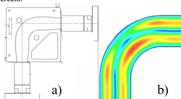
Figure 3: a) High-power TE_{01} bend with converters and b) electric field plot of interior overmoded rectangular H-plane bend.
