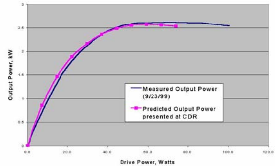
Figure 4: VKP-8290A Transfer Curve
