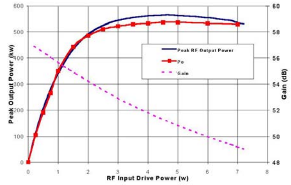
Figure 6: VKP-8291A Transfer Curve
