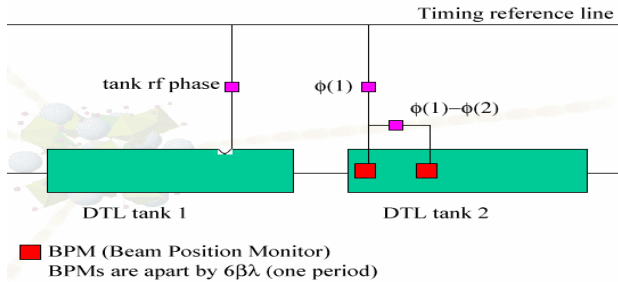
Figure 1: Schematic plot of phase scan with two downstream BPMs.
