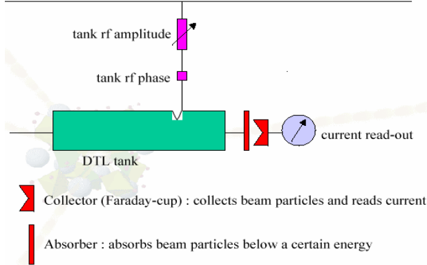
Figure 4: Schematic drawing of acceptance scan with the absorber and collector.
