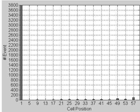
Figure 6 Breakdown locations in traveling wave structure
