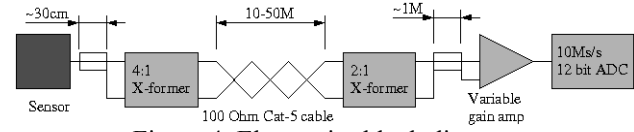
Figure 4: Electronics block diagram
