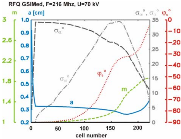
Figure 2: Design parameters of the RFQ.
