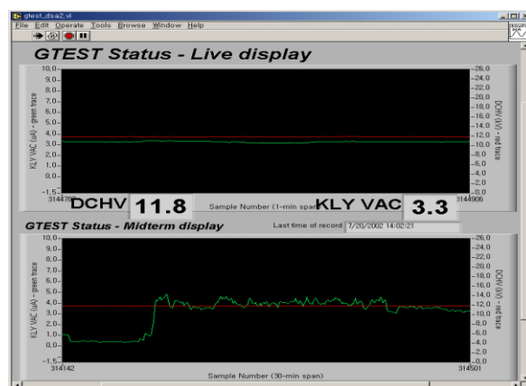
Figure 7: Historical real time trend view of HV&Vacuum signal
