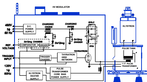
Figure 1: Simplified circuit diagram of the K&M system
