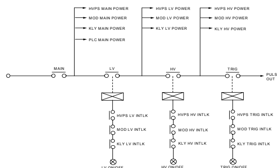
Figure 2: Simplified control sequence of the K&M system
