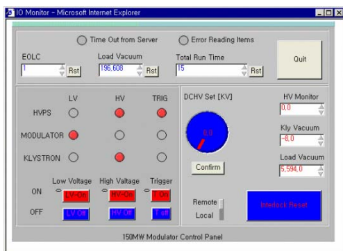
Figure 6: Main control panel through MS Explorer
