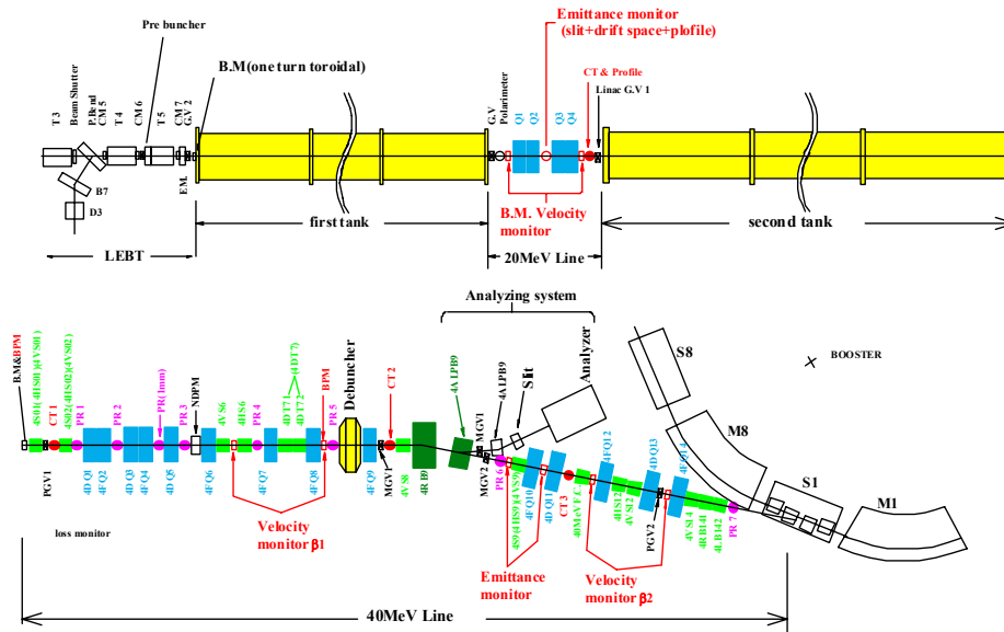
Fig.2: KEK PS-40 MeV proton linac and the 40 MeV beam line
