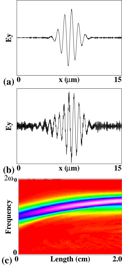
Figure 2: One-dimensional simulation results : (a) the pulse shape at the initial time, (b) the pulse shape when the interaction length is 2 cm, and (c) contour plot of frequency vs. interaction length.
