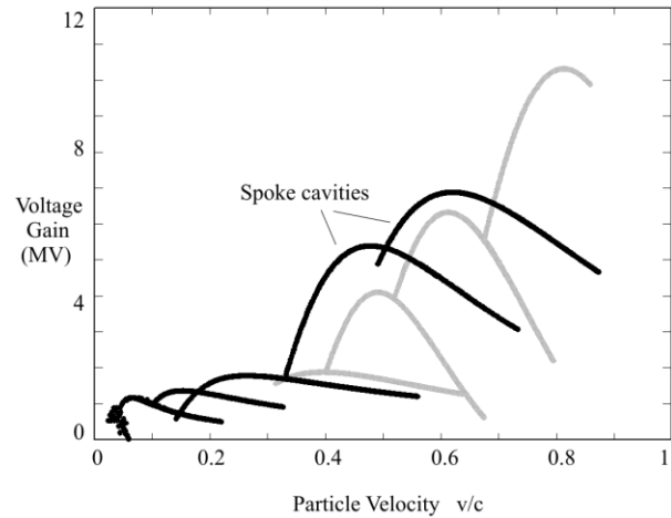
Figure 4: Voltage gain/cavity along the linac for the spoke-cavity option (elliptical-cell option is shaded). Plots for several ion species are overlaid to show the full velocity range required of each cavity type.
