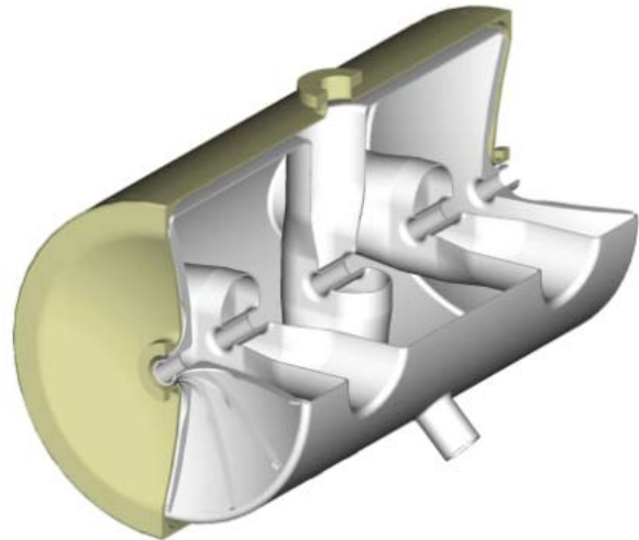
Figure 3: Section view of an 85 cm long, 345 MHz, triple-spoke-loaded niobium cavity for \beta = 0.62
