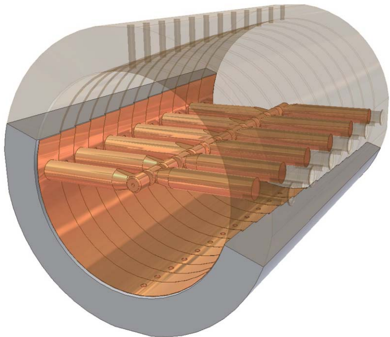
Fig. 1. An Interdigital Configuration for the RFI Linac.
