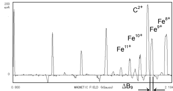
Figure 3: Charge spectrum in producing Fe ions with the 18GHz-ECRIS
