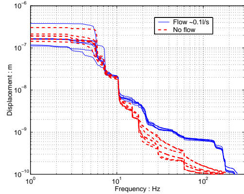
Figure 8: Integrated Displacement Spectrum of the water induced vibration in the EM quadrupole at nominal flow. The region below 10Hz is disturbed by resonances of the concrete table installed on rubber pads.
