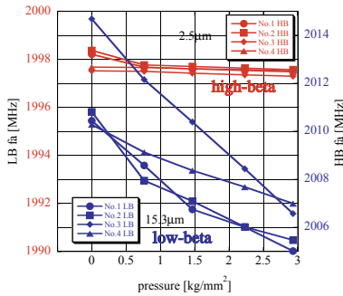
Figure 3: Effect of flatness on frequency shift
