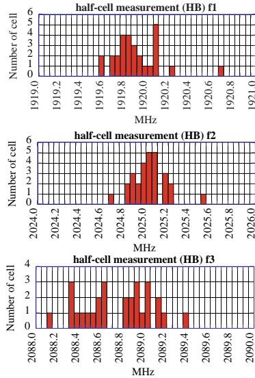
Figure 5: Frequency distribution of 28 half-cells (high-beta model)
