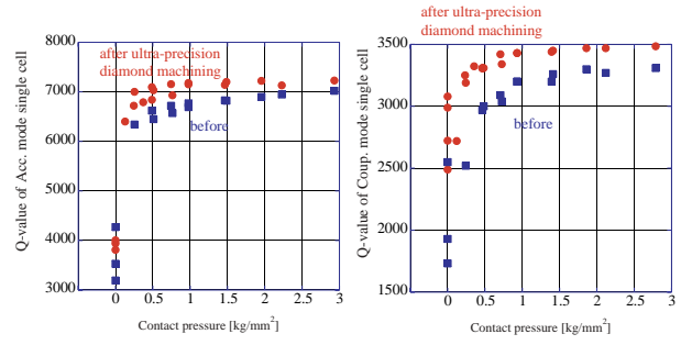
Figure 4: Q-value and Contact pressure
