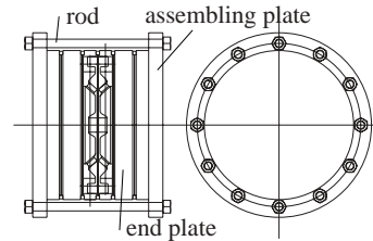
Figure 2: Whole view of the measurement setup
