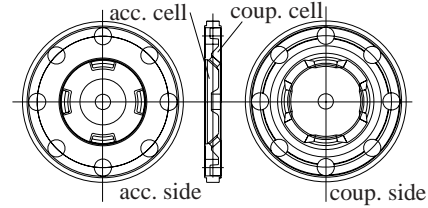
Figure 1: Configuration of the half-cell disk
