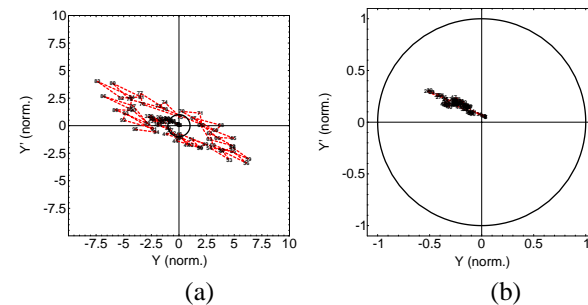
Figure 4. Phase Space (3MHz RMS error). The phase space to the left (a) is for a linac composed of 4720 structures assumed to have identical random errors in each structure. The phase space to the right (b) has been computed from a linac composed of structures with a different random error in the synchronous frequency (non-identical structures).
