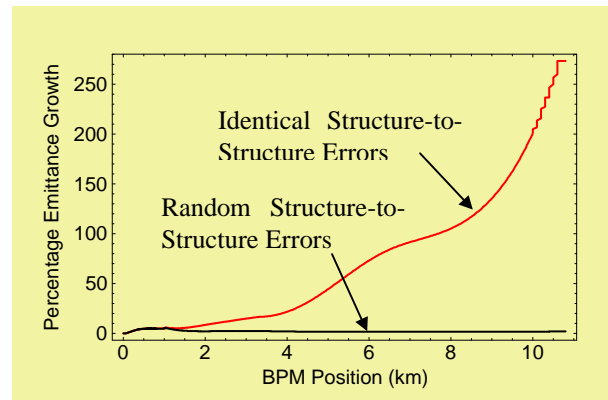
Figure 3. Emittance growth due to 3MHz RMS errors that are (a) reproduced in every structure and (b) random from structure-to-structure.
