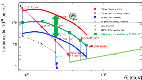
Figure 3: Luminosities for various options for a high-energy e^+e^- collider. The plot was taken from [9]. Three CERC luminosity curves are added in blue, green, and red added to it for levels of synchrotron radiation power of 10 MW, 30 MW, and 100 MW, respectively.
