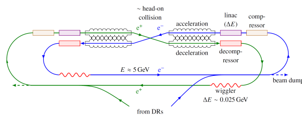
Figure 4: ERLC: A re-imagining of the ILC as an ERL.
